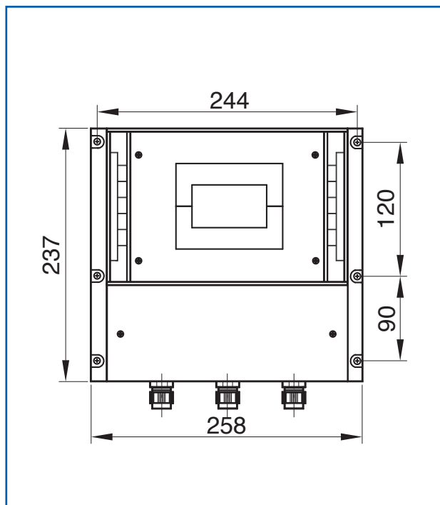
Fig. 4: Field electronics (PME) dimensions
