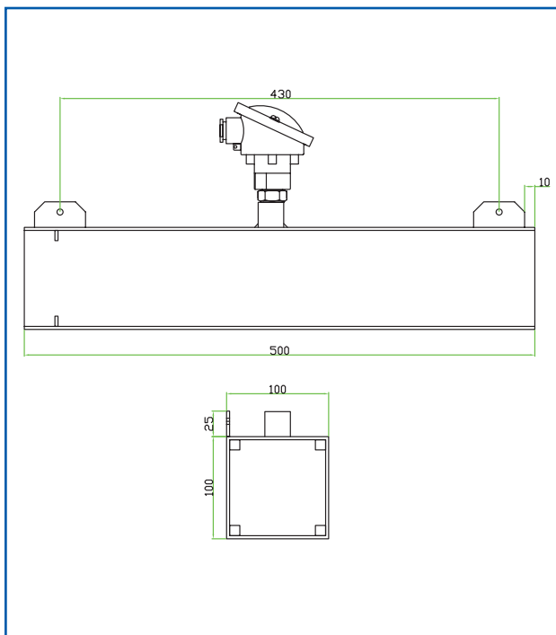
Fig. 3: AirSafe dimensions
