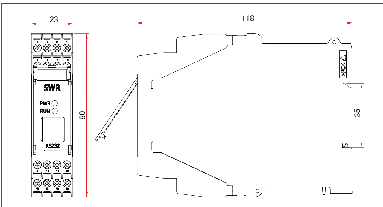
Fig. 5: DIN rail transmitter dimensions
