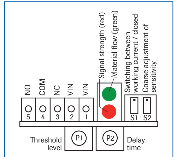
Fig. 11: Position of operating controls
