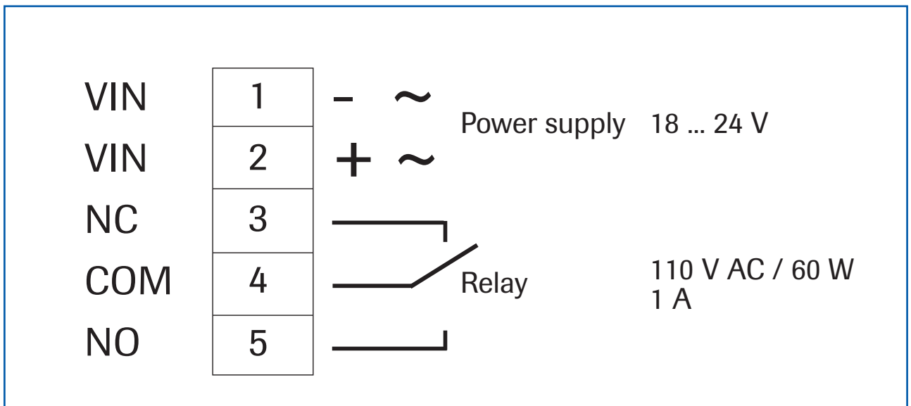
Fig. 10: Wiring diagram for sensor
