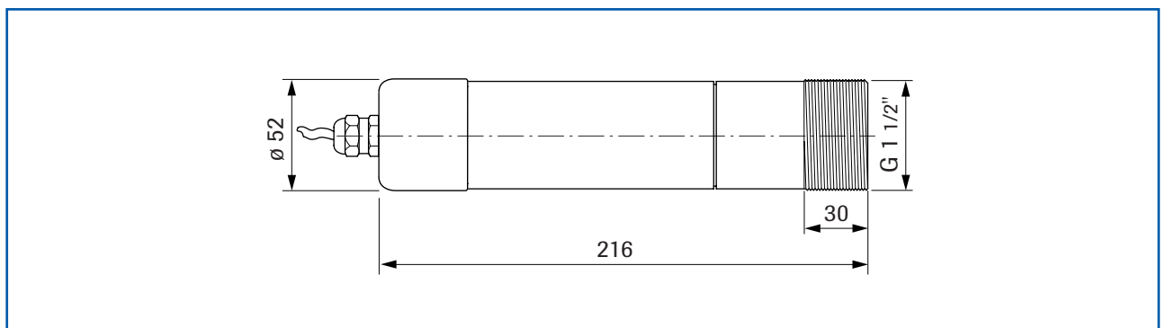
Fig. 2: Dimensioned drawing
