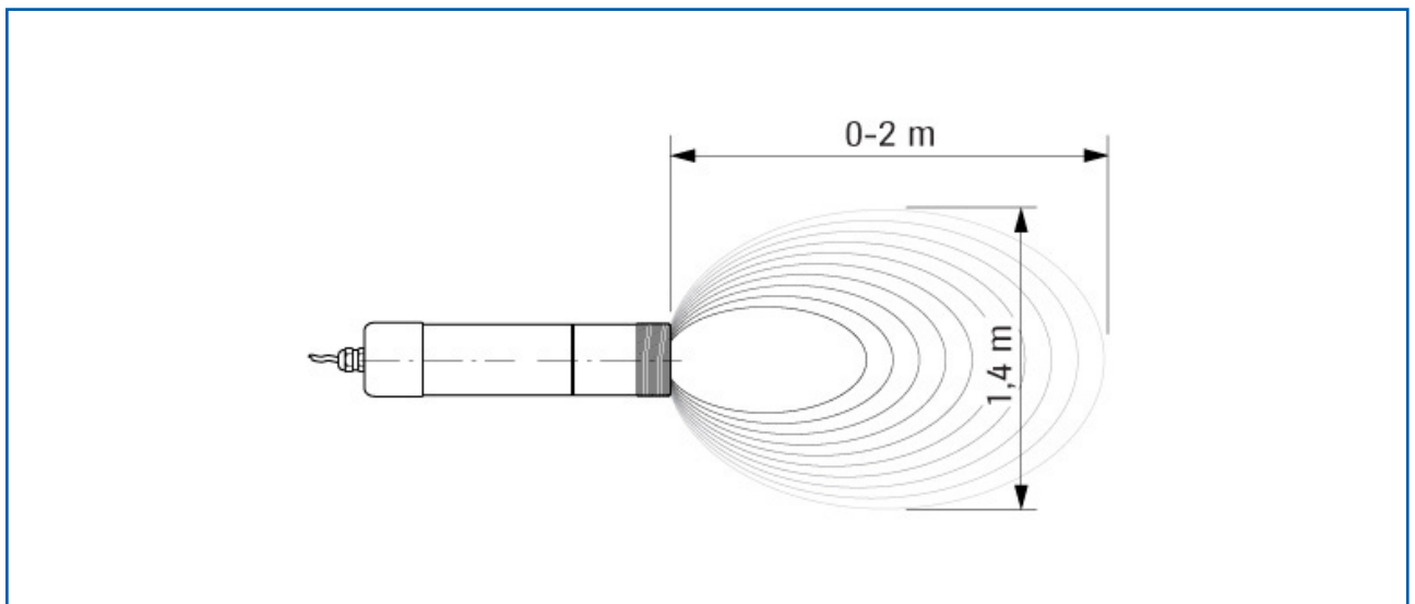
Fig. 1: Detection range
