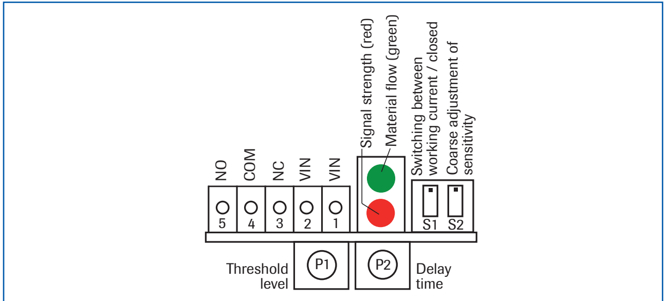
Fig. 9: Terminal and operational controls
