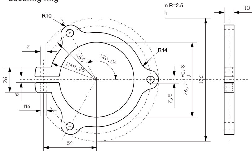
Base flange
